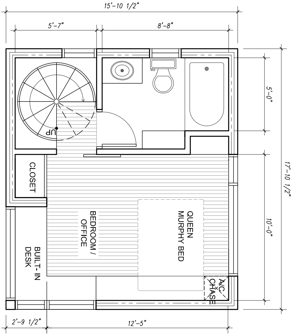
SECOND FLOOR PLAN 248 SF
