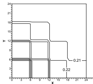
FIG. 10. Coarse-scale saturation at 20 days for Example 2.
